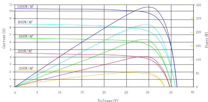
Current-Voltage&Power-Voltage Curver
